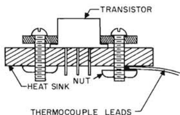
THERMOCOUPLE PLACEMENT
