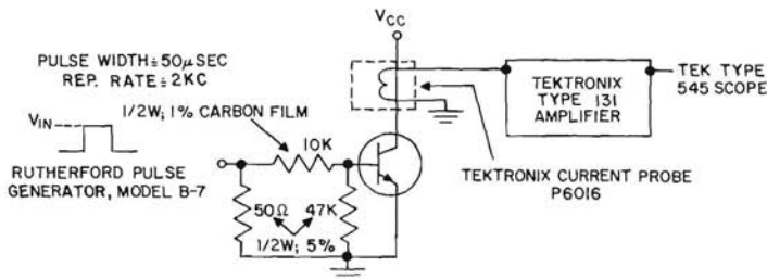
\tau_a TEST CIRCUIT
