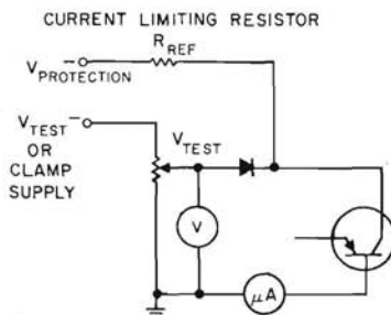
COMPLETE I_{CBO} TEST CIRCUIT
