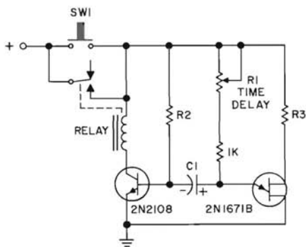
DELAYED DROPOUT RELAY TIMER
