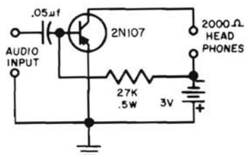
SIMPLE AUDIO AMPLIFIER Figure 15.1
