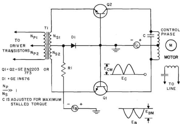
GROUNDING BASE SERVO OUTPUT STAGE
