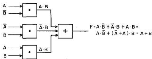
(a) F = A + B IN UNSIMPLIFIED FORM
