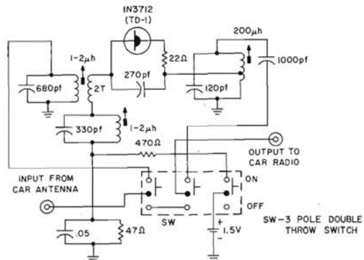
CIVIL AIR PATROL CONVERTER (A)
