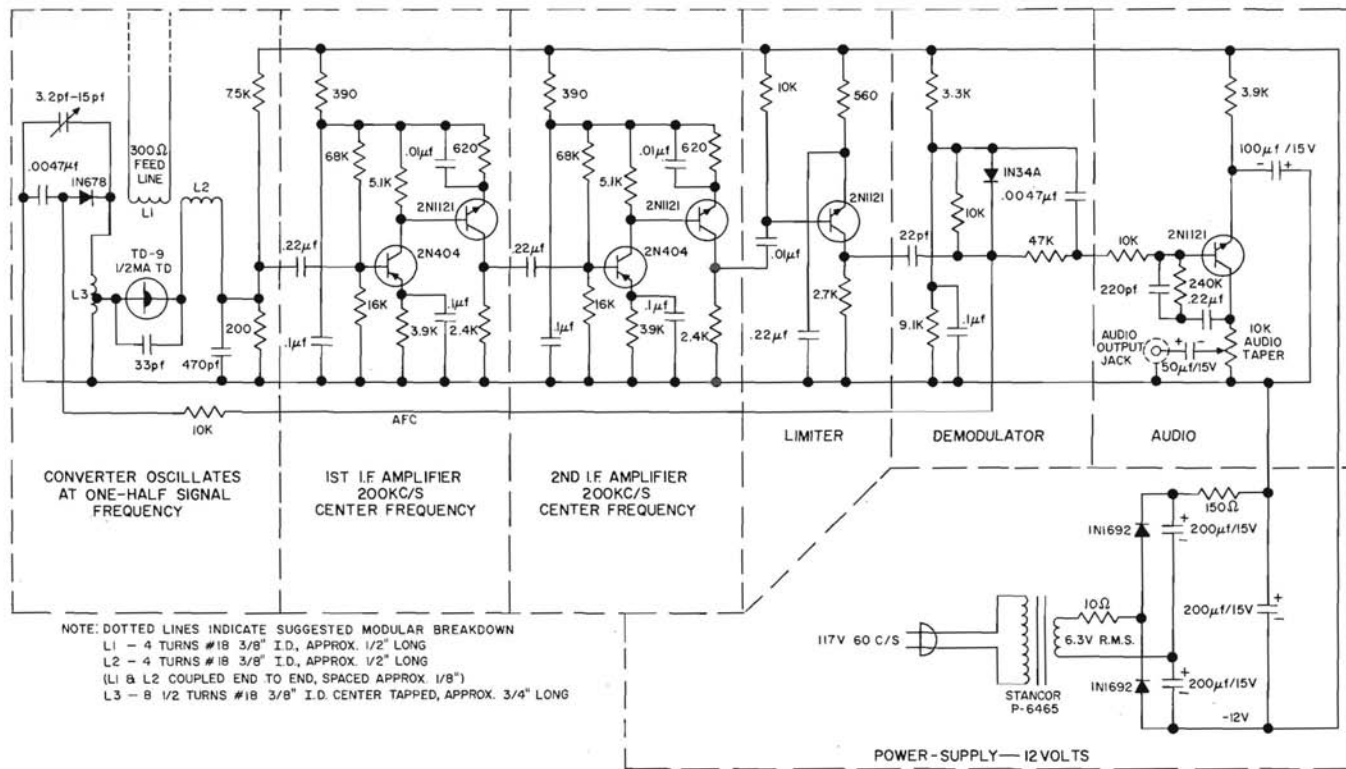
FM BROADCAST BAND TUNER (88 to 108 MC)
