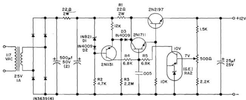
PRECISION REGULATED VOLTAGE SUPPLY
