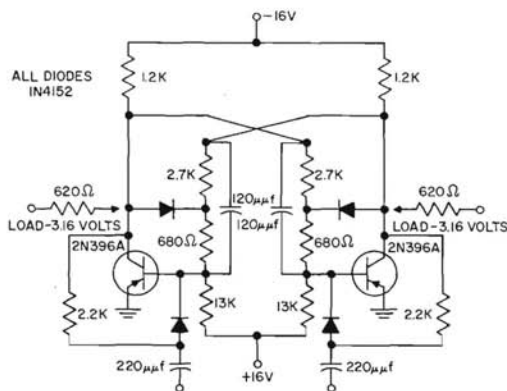
NON-SATURATED FLIP-FLOP Figure 7.10 (B)
