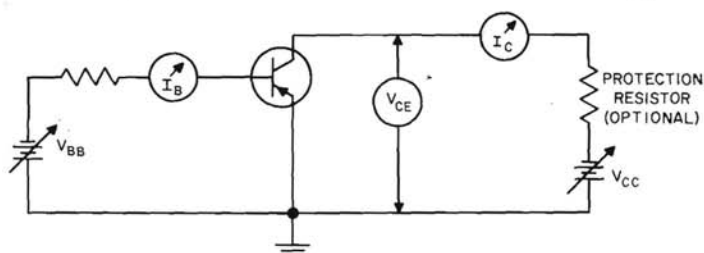
h_{FE} MEASUREMENT
