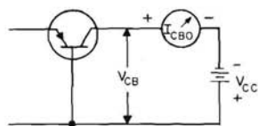
I_{CBO} MEASUREMENT
