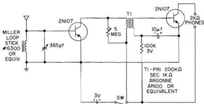
TWO TRANSISTOR RECEIVER (AM Broadcast Band)
