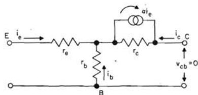
(A)-COMMON-BASE
