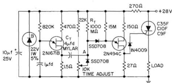
ONE HOUR TIME DELAY CIRCUIT
