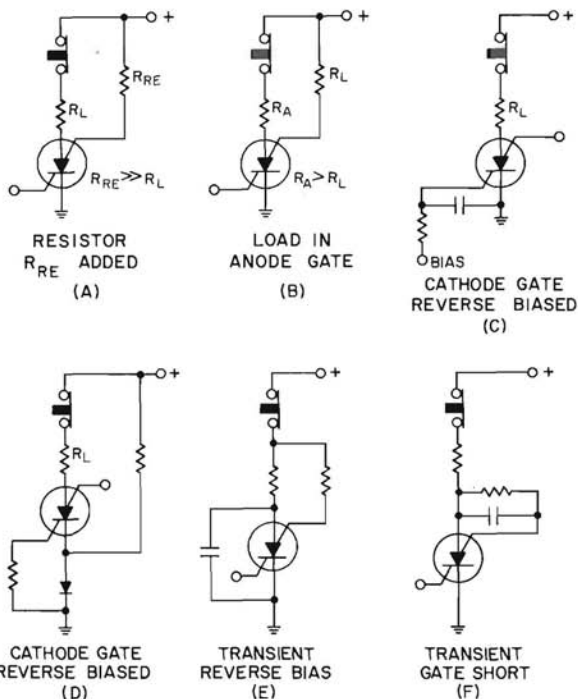
MINIMIZING RATE EFFECT Figure 16.20
