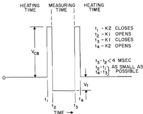
OSCILLOSCOPE PATTERN
