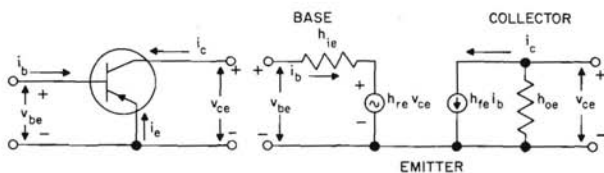
(B)-COMMON-EMITTER
