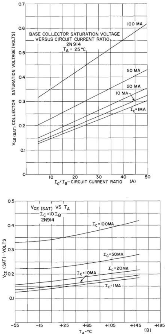
VARIATIONS IN V_{CE(SAT)} WITH TEMPERATURE, COLLECTOR CURRENT, AND FORCED GAIN
