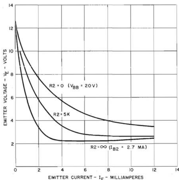
EMITTER CHARACTERISTIC CURVES FOR TYPE 2N492 UNIUNCTION TRANSISTOR WITH BASE-TWO SERIES RESISTANCE
