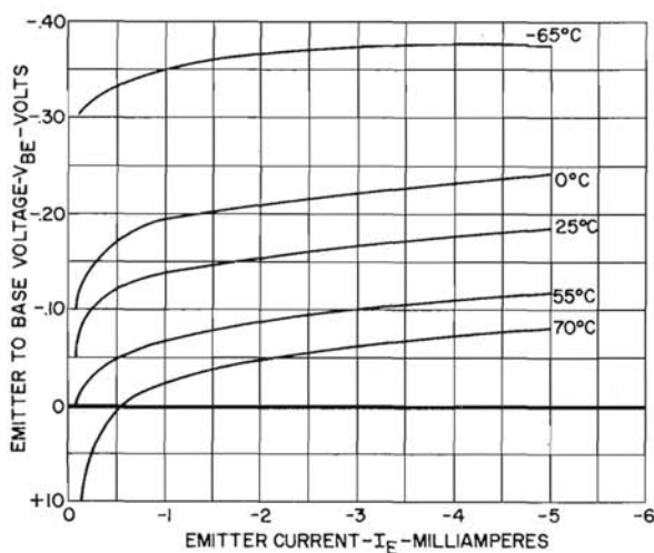
INPUT CHARACTERISTICS OF 2N525 ( V_{CE} = 1V )
