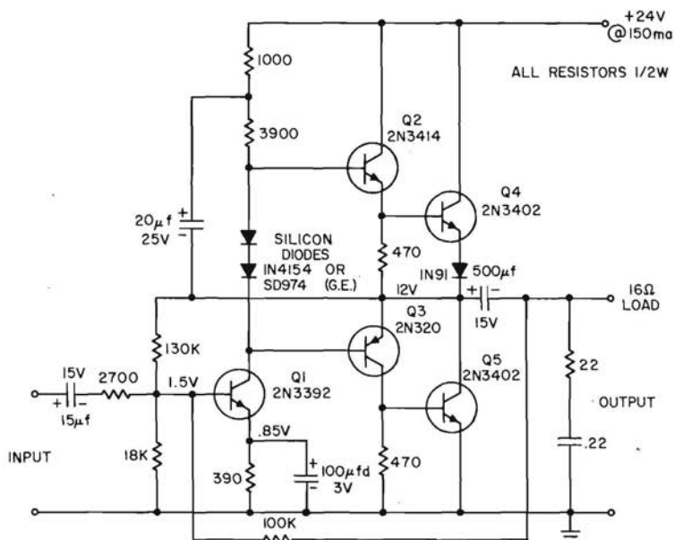
2½ WATT AMPLIFIER
