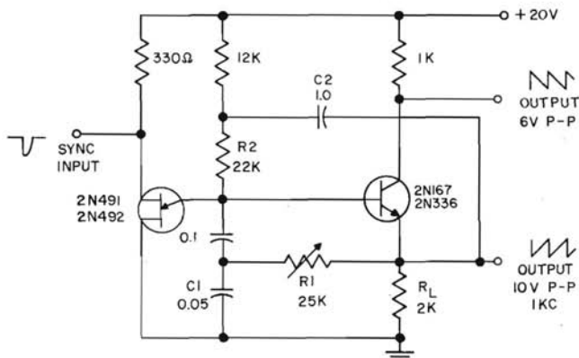
SAWTOOTH GENERATOR WITH HIGH LINEARITY Figure 13.28
