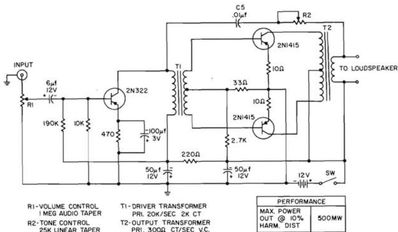
12 VOLT AUDIO AMPLIFIER Figure 11.6
