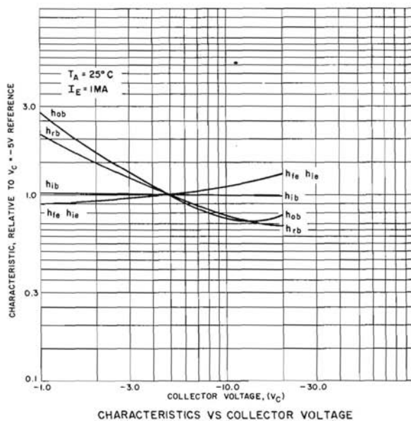
VARIATION OF h-PARAMETERS WITH BIAS CONDITIONS
