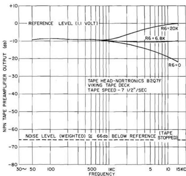
TAPE PREAMPLIFIER RESPONSE FROM NAB RECORDING Figure 11.23
