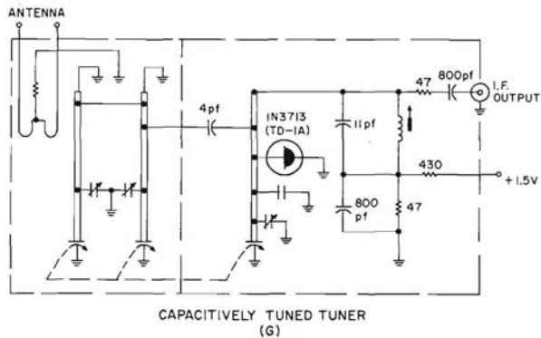
Figure 14.20 SELF-OSCILLATING TUNNEL DIODE CONVERTERS
