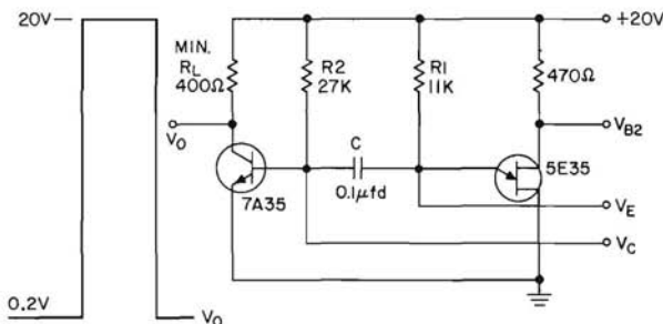
TRANSISTOR-UJT MULTIVIBRATOR
