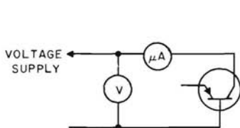
BASIC I_{CBO} CIRCUIT
