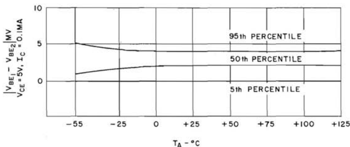
(a) V_{BE} MATCH VS. TEMPERATURE FOR 2N2480
