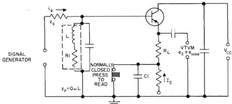
Figure 18.38 h_{re} MEASUREMENT
