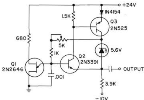
50 KC SAWTOOTH GENERATOR Figure 13.27
