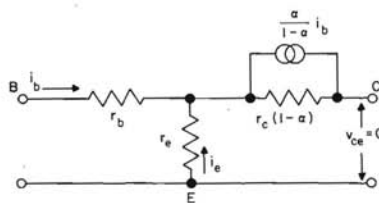
(B)-COMMON-EMITTER
