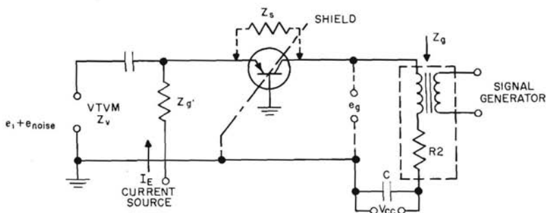
h_{rb} MEASUREMENT
