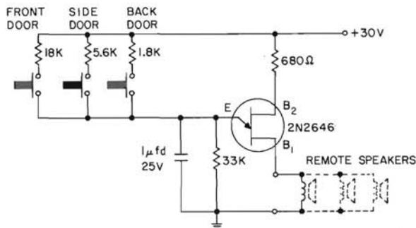
UNIUNCTION HOME SIGNAL SYSTEM
