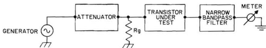
SET UP TO MEASURE (\overline{e_N^2})^{1/2} Figure 18.60
