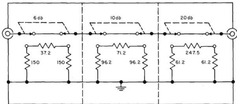
Figure 18.52 ATTENUATOR BOX
