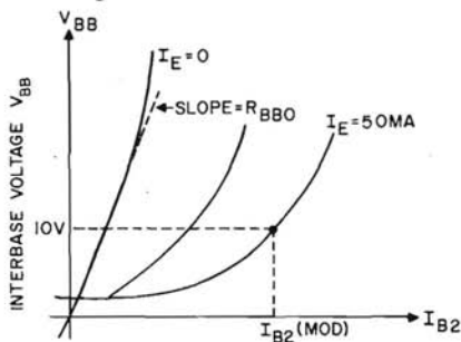
BASE-TWO CURRENT STATIC INTERBASE CHARACTERISTICS CURVES
