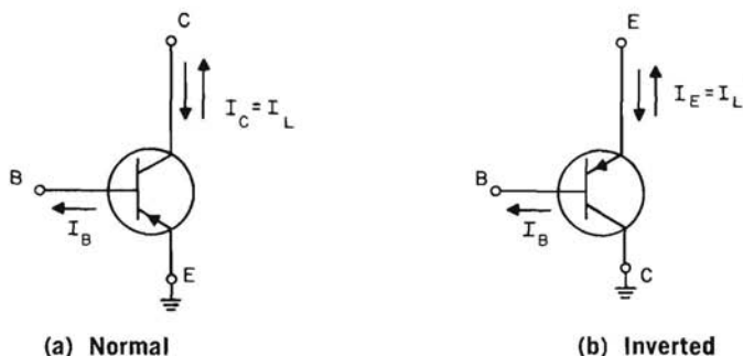
THE NORMAL AND INVERTED CONNECTIONS
