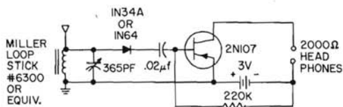
ONE TRANSISTOR RECEIVER (AM Broadcast Band)
