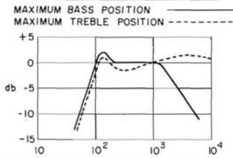
FREQUENCY RESPONSE OF FOUR TRANSISTOR AMPLIFIER
