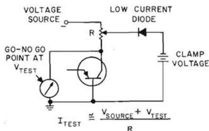
GO-NO GO I_{CBO} TEST CIRCUIT
