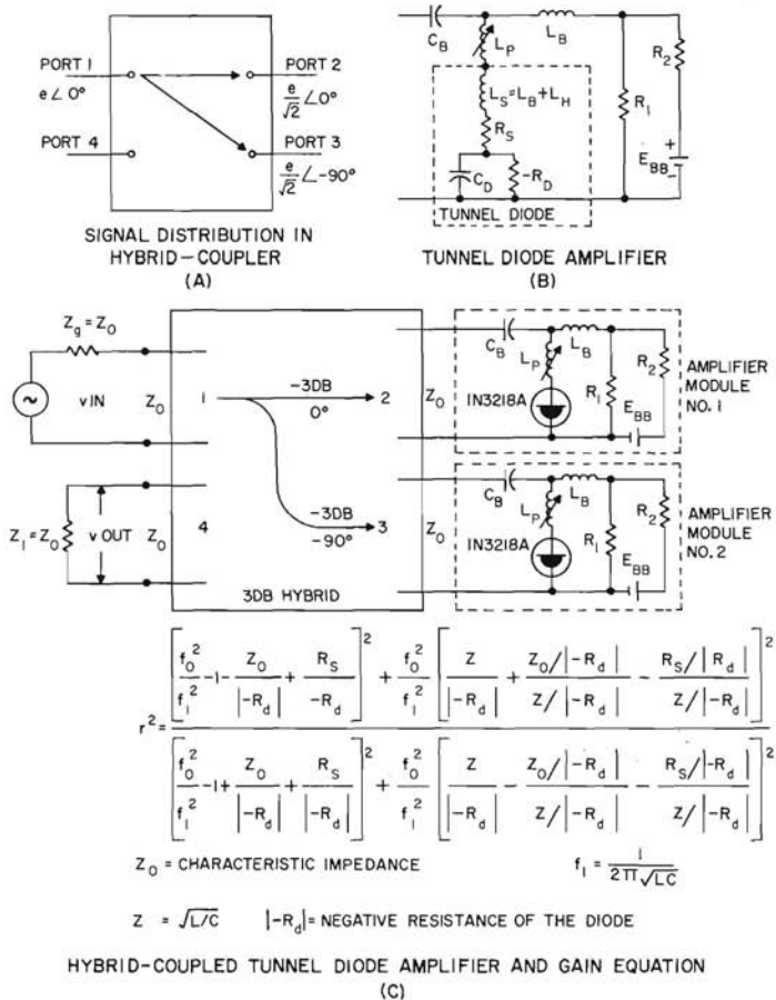
Figure 14.31 TUNNEL DIODE SIX-GIGACYCLE WAVEGUIDE AMPLIFIER
