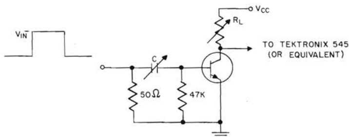
Q_B^* TEST CIRCUIT
