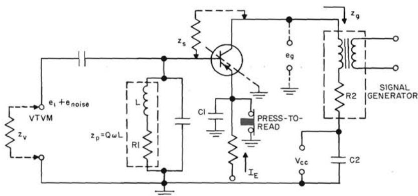
h_{re} MEASUREMENT
