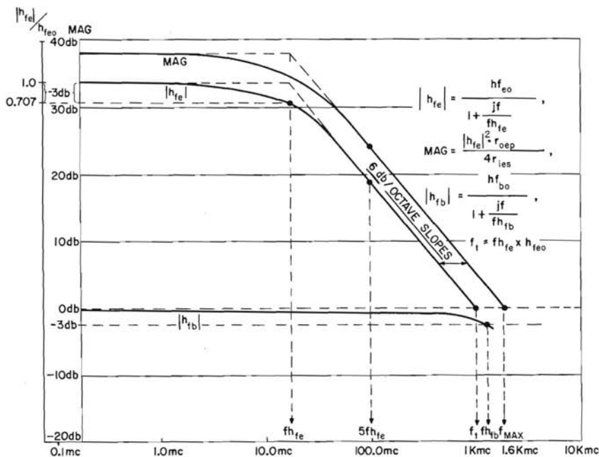
MAG, |h_{fe}| , |h_{rb}| VS. FREQUENCY OF TYPICAL UHF TRANSISTOR
