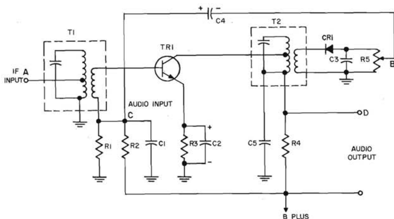
REFLEX IF-DETECTOR CIRCUIT
