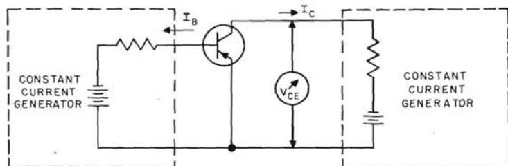
GO-NO GO h_{FE} CIRCUIT
