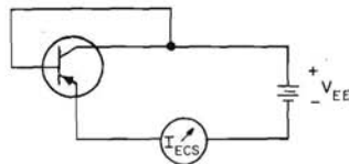
I_{ECS} MEASUREMENT
