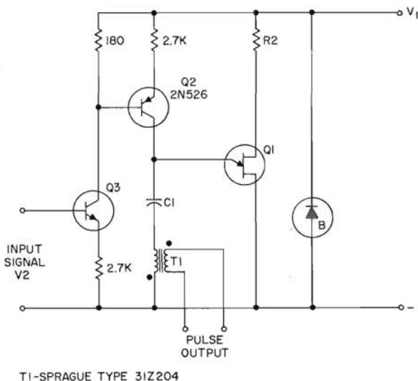
SERIES TRANSISTOR CONTROL OF UJT Figure 13.52
