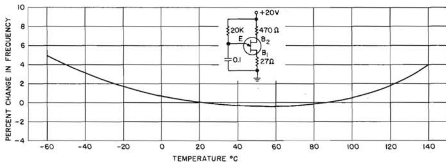
UNIUNCTION ONLY SUBMITTED TO TEMPERATURE
