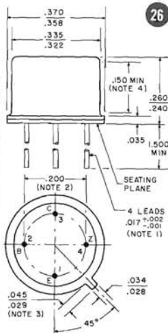
DIMENSIONS WITHIN JEDEC OUTLINE TO-12
