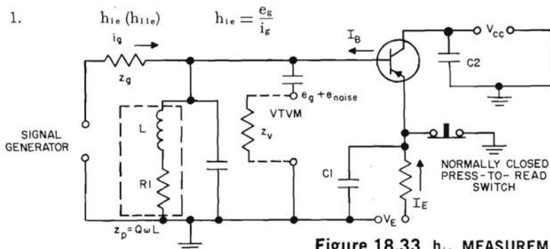
Figure 18.33 h_{ie} MEASUREMENT
