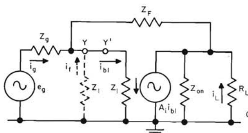
(B) SIMPLIFIED EQUIVALENT CIRCUIT
