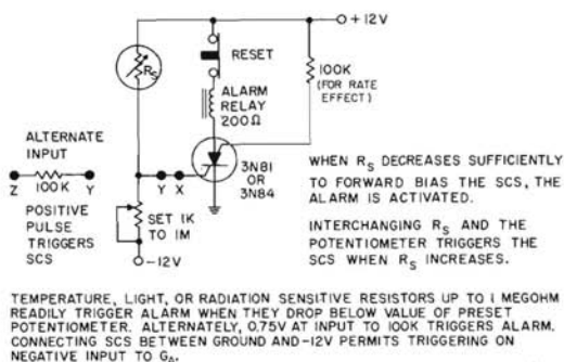
(A) ALARM CIRCUIT
