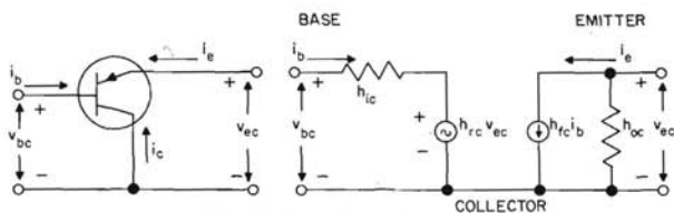
(C)-COMMON-COLLECTOR
