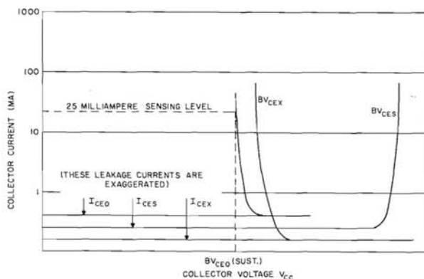
TYPICAL PLANAR EPITAXIAL COLLECTOR BREAKDOWN CHARACTERISTICS
