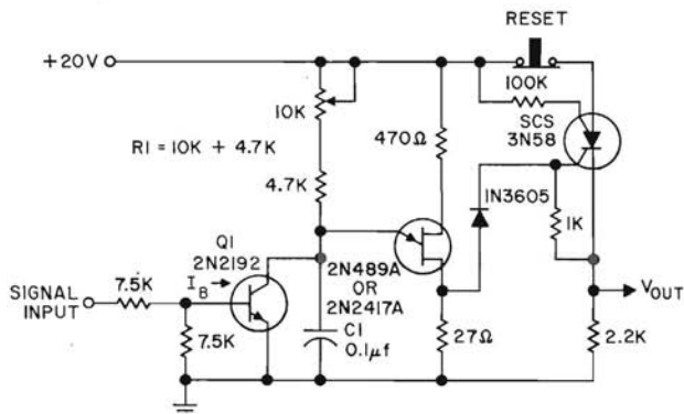
SIGNAL DROPOUT DETECTOR
