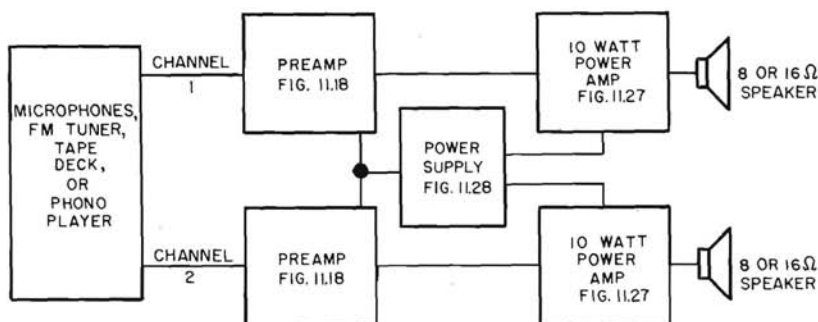
BLOCK DIAGRAM OF 20 WATT STEREO SYSTEM
