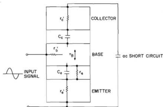
VARIOUS TIME-CONSTANTS LIMITING THE GAIN-BANDWIDTH PRODUCT OF THE TRANSISTOR
