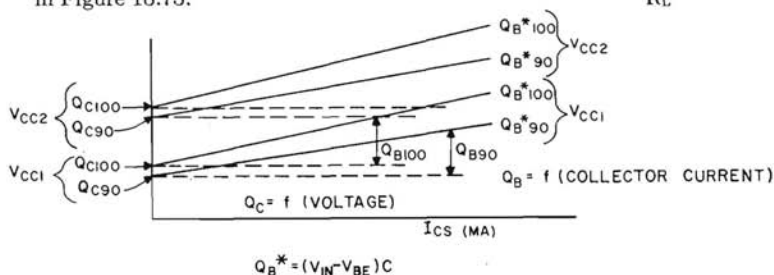
Q_B^* PLOT VS. I_{CS}
