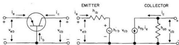
(A)-COMMON-BASE
