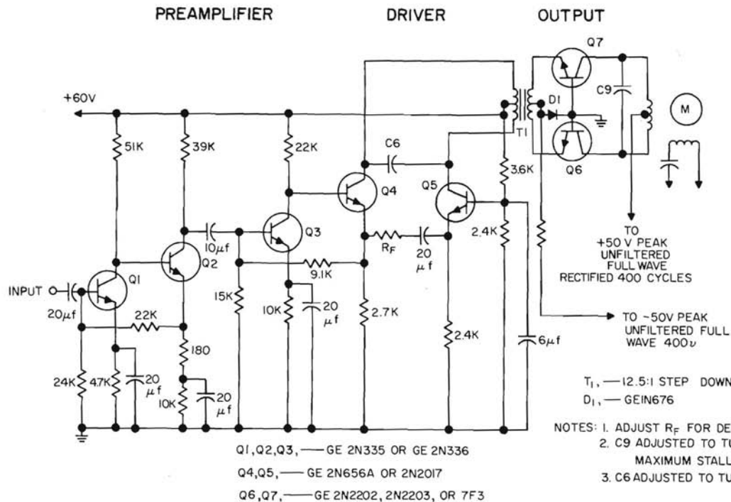
3 WATT 400 CYCLE SERVO AMPLIFIER FOR -55°C TO 125° OPERATION
