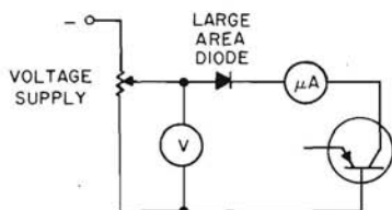
I_{CBO} CIRCUIT WITH METER PROTECTION
