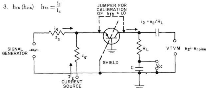
Figure 18.31 h_{fb} MEASUREMENT
