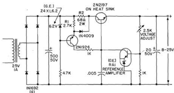
GENERAL PURPOSE POWER SUPPLY WITH CURRENT LIMITING
