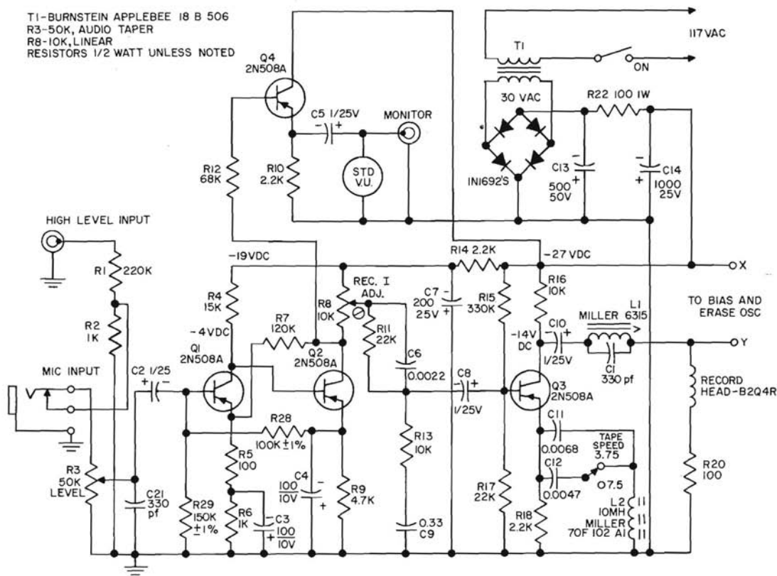
Figure 11.54 RECORDING AMPLIFIER
