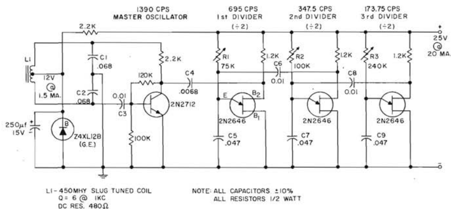
UNIUNION FREQUENCY DIVIDER
