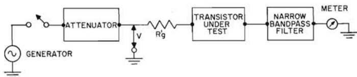
Figure 18.61 SET UP TO MEASURE (\bar{i}_N^2)^{1/2}
