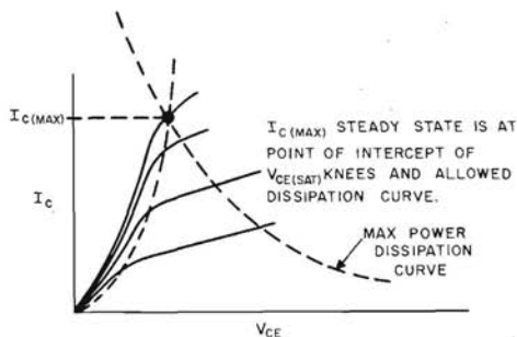
I_C(MAX) STEADY STATE
