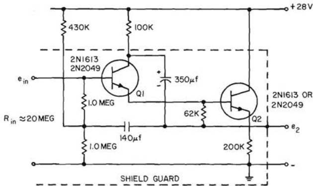
BOOTSTRAPPED EMITTER FOLLOWER
