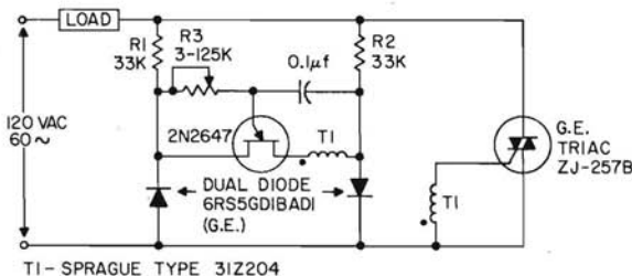
UJT/TRIAC PHASE CONTROL
