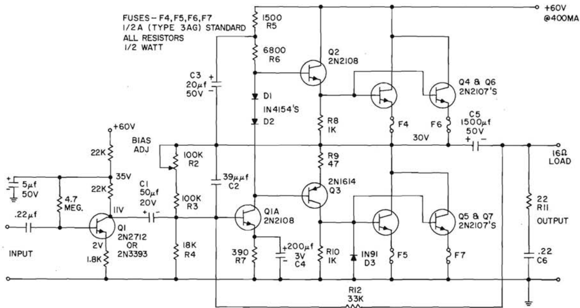
15 WATT AMPLIFIER Figure 11.40
