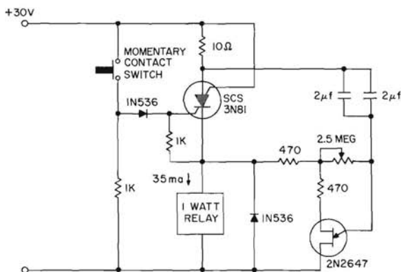
10 SECOND TIMER.
