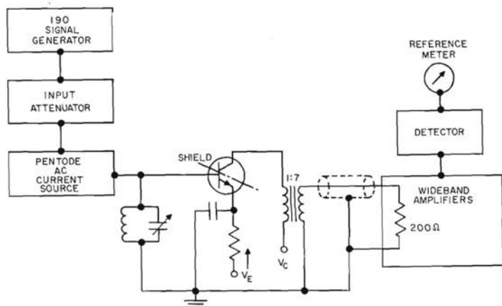
h_{fe} AND f_{ce} MEASUREMENT UP TO 10 MCS
